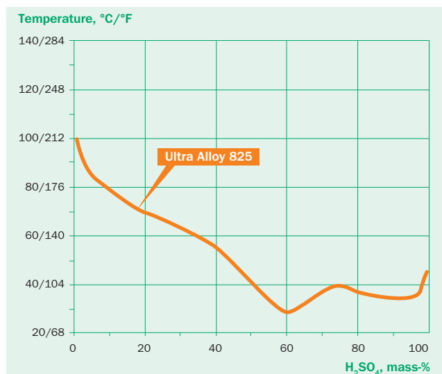
Fig. 1. Isocorrosion diagram in naturally aerated sulphuric acid of chemical purity, based on uniform corrosion tests with sample activation according to ISO 18069. The line represents a limit for corrosion resistance, below which the corrosion rate is lower than 0.1 mm/year.
